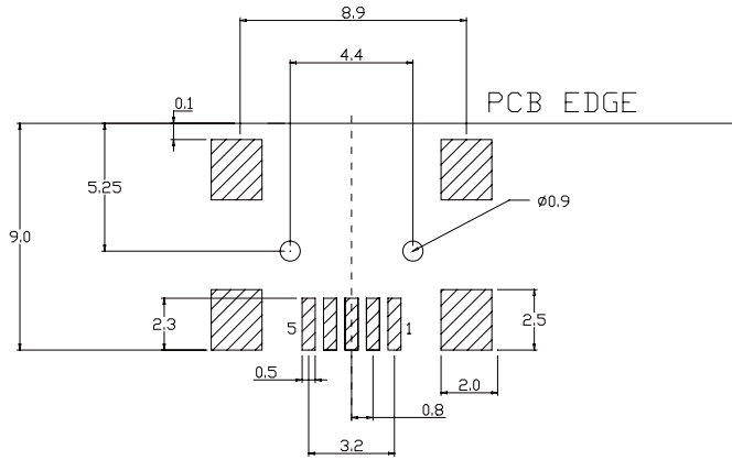
RECGMENDED PCB PATTERN LAYOUT
